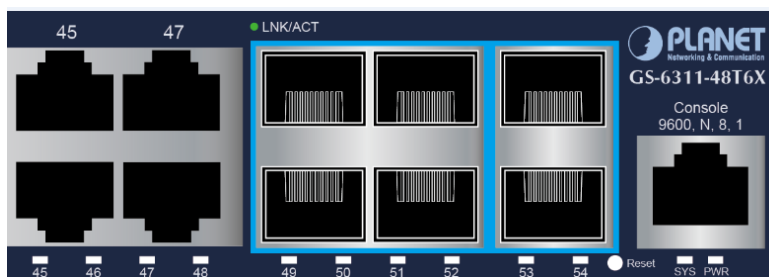
Figure GS-6311-48T6X front panel
