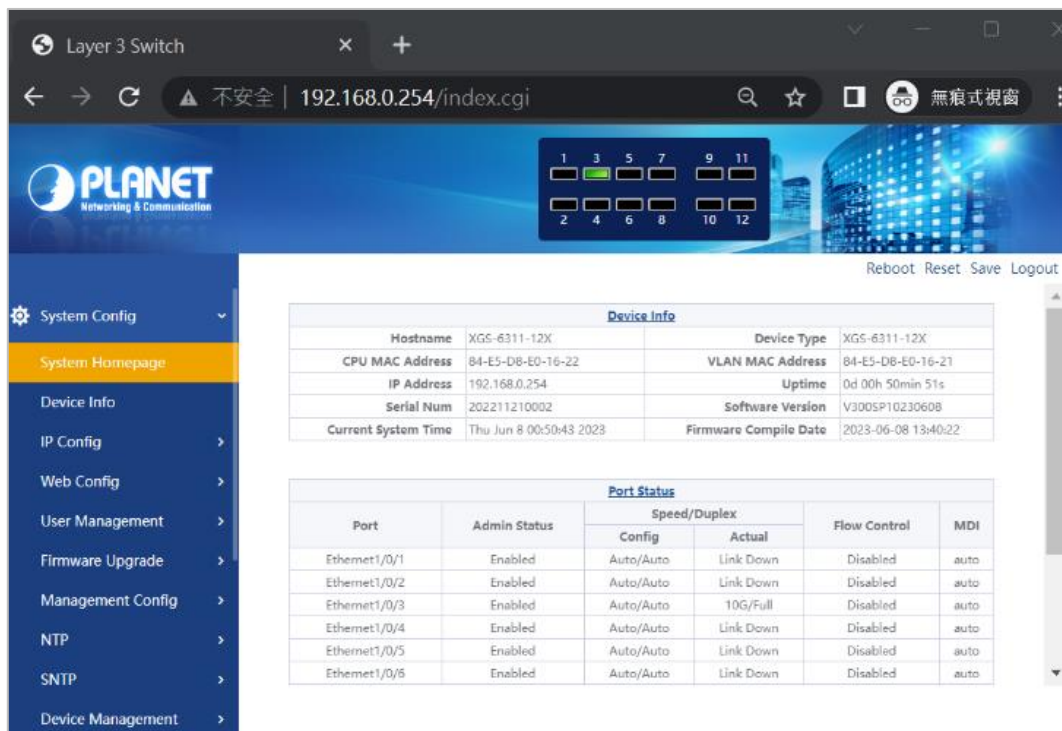
Figure 5-5 Web Main Screen of Managed Switch
