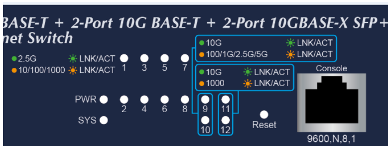
Figure MGS-6311-10T2X front panel
